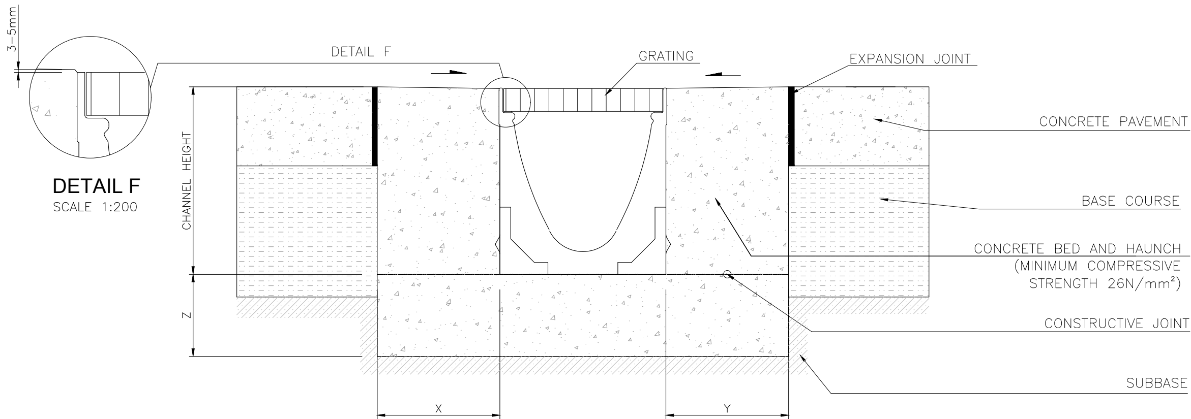
INSTALLATION DETAIL IN CONCRETE PAVEMENT FOR LOAD CLASS C250
