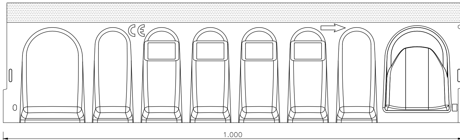
POLYMER CONCRETE CHANNEL WITH GRATING COVER w=0.15\text{ m} (SLOPING DEPTH)
