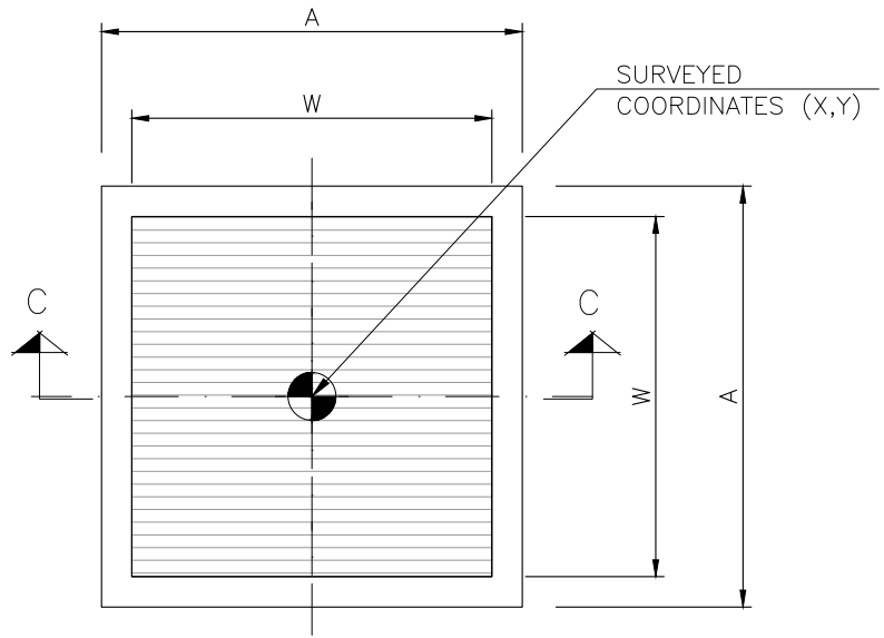
PLAN VIEW DETAIL SUMP COVER
